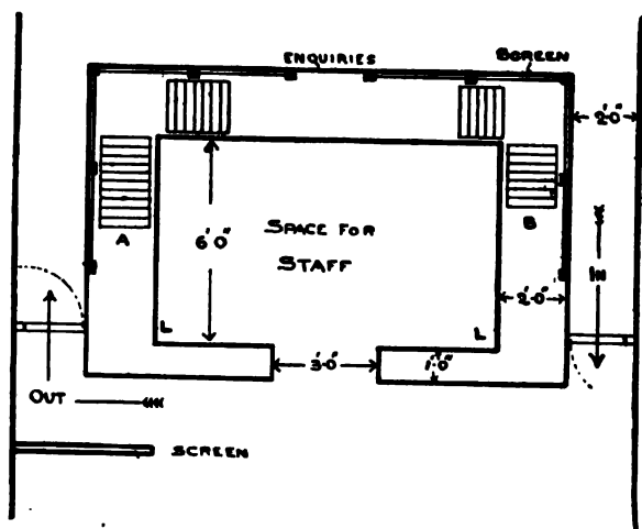
FIG. 25.—Single Open-Access Barrier (Section 160).
